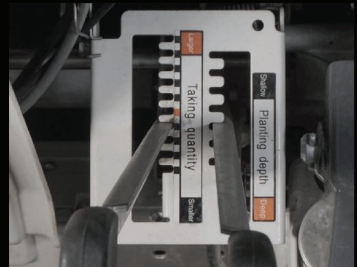
Planting depth adjustment lever
