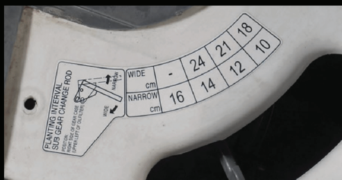
Hills space adjusting lever
